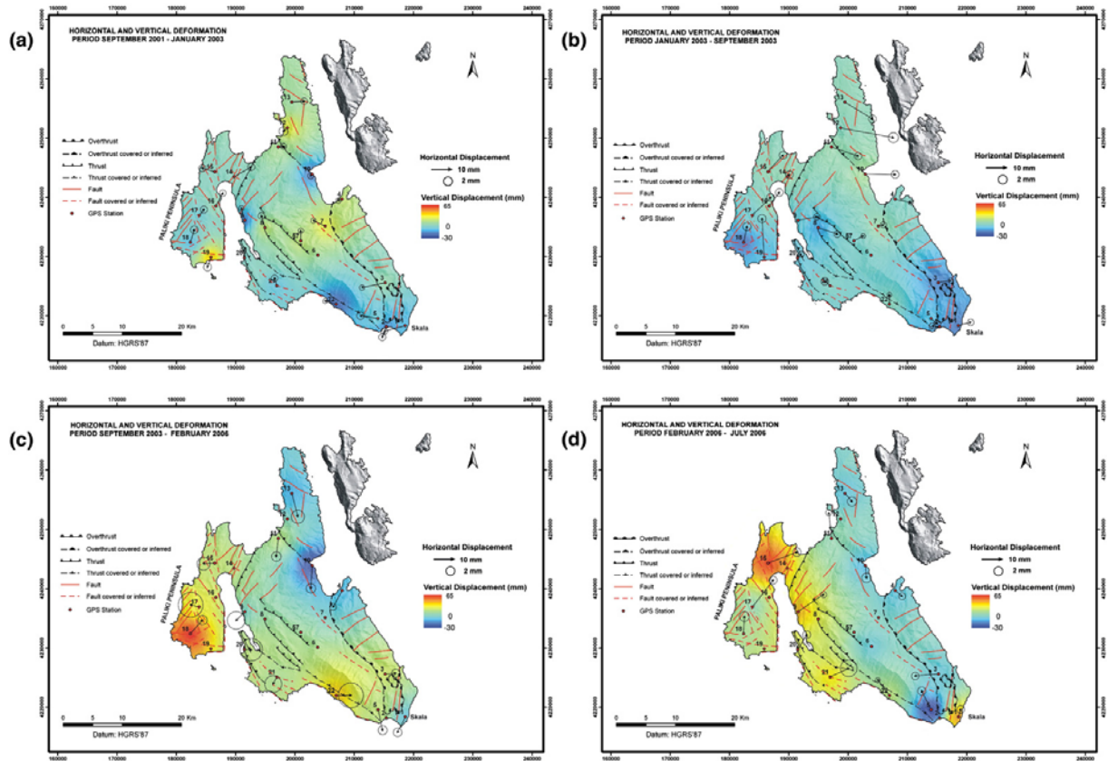
Fig. 6. DGPS results from the Cephallonian network relative to station No. 06 (Aenos Mt.) for various observational periods, (a) Sept. 2001 to Jan. 2003; (b) Jan. 2003 to Sept. 2003; (c) Sept. 2003 to Feb. 2006; and (d) Feb. 2006 to July 2006.
